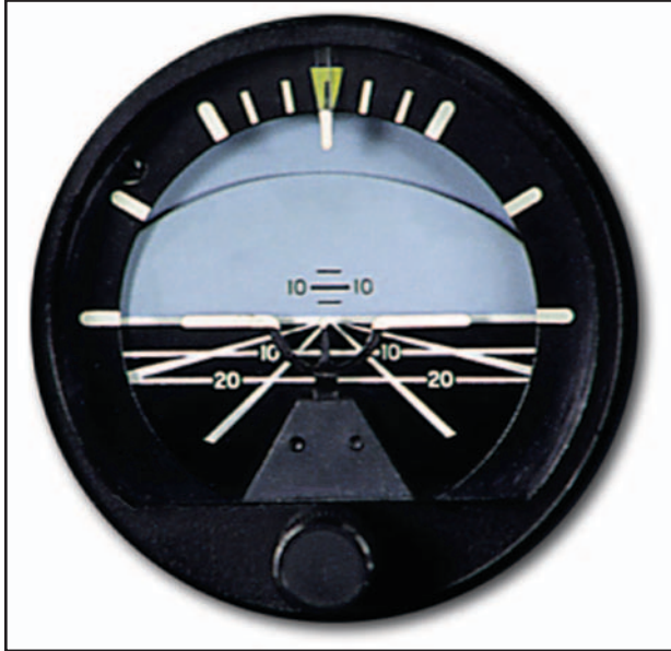
Figure 16-11. Attitude indicator.
