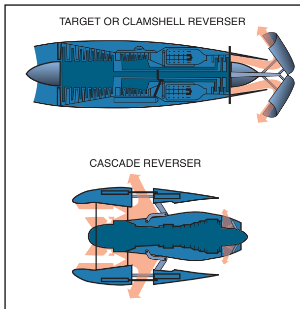
Figure 15-19. Thrust reversers.
