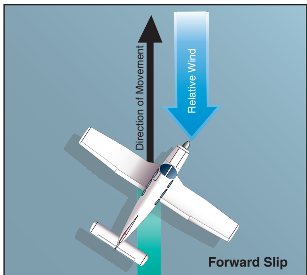
Figure 8-13. Forward slip.
